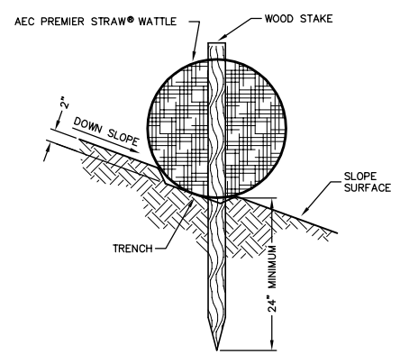
STAKE DETAIL (ON BARE SOIL) NO SCALE
