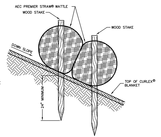
STAKE DETAIL (SECTION VIEW) NO SCALE
