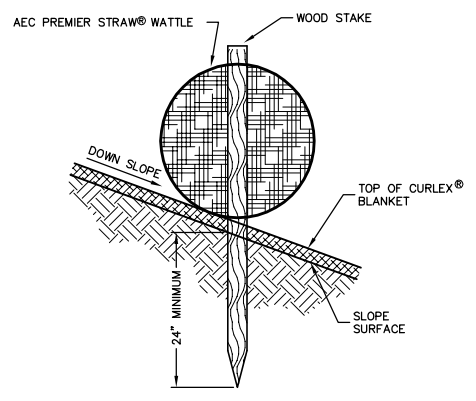
STAKE DETAIL (ON TOP OF CURLEX® ECB) NO SCALE
